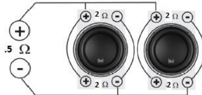
(2) 2ohm DVC Speaker = .5 ohm Load
