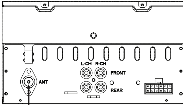
Antenna Connector
