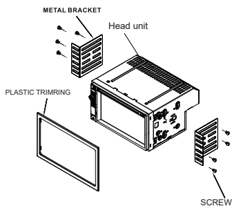
Fig 3 Installation to use the Metal Brackets. (Included)
