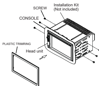
Fig 2 Once the unit is inserted into the kit, secure the head unit with the supplied screws
