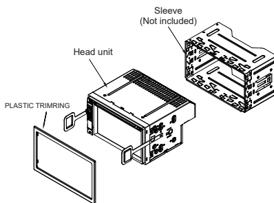
Fig 4 Installation to use the sleeve.
