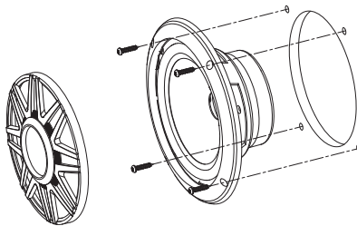
TYPICAL MOUNTING
